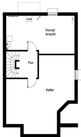
Plan subsol
