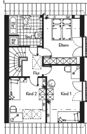
Plan mansarda
