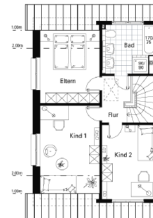
Plan mansarda
