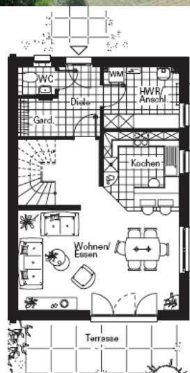
Plan parter
