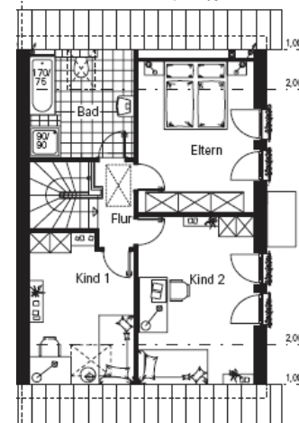
Plan mansarda
