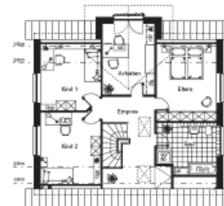
Plan mansarda
