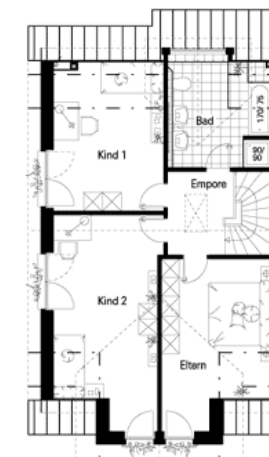
Plan mansarda
