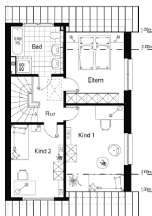
Plan mansarda
